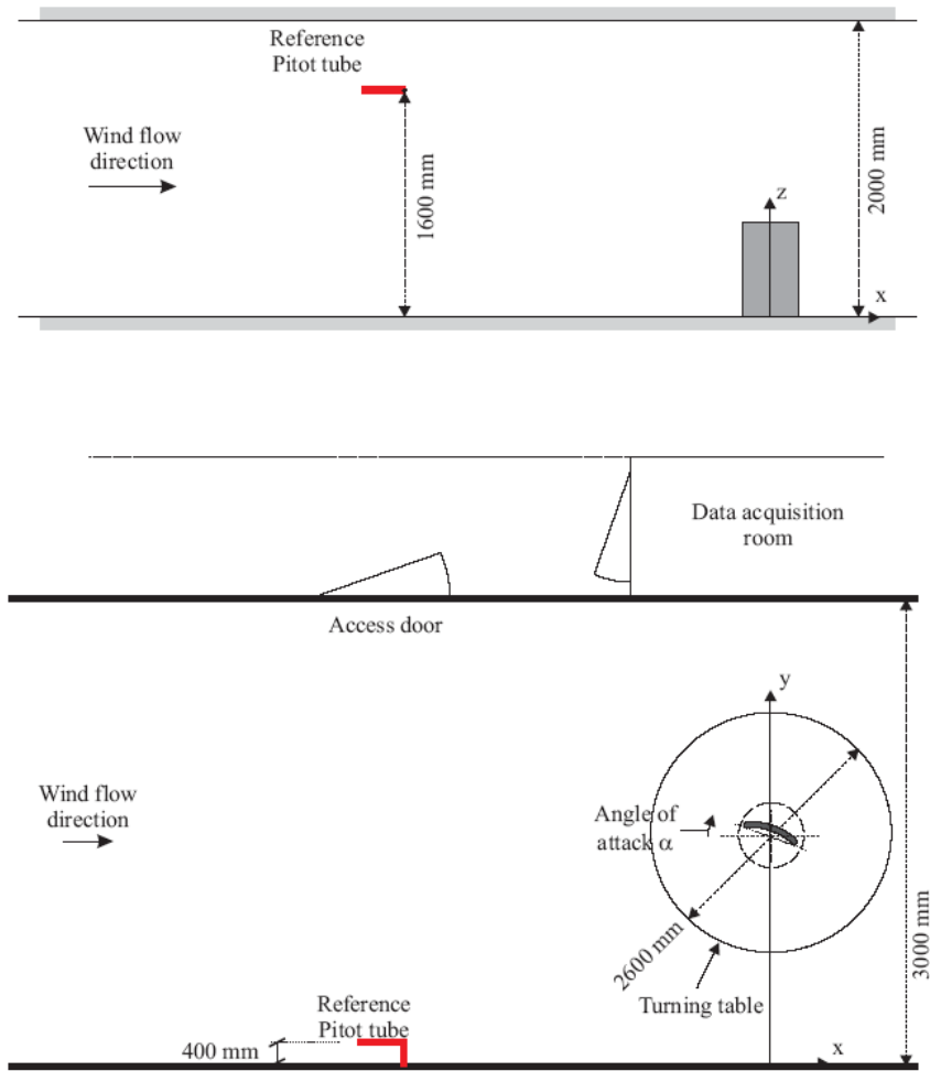
Fig. 2-1 - Sketch of the wind tunnel setup
