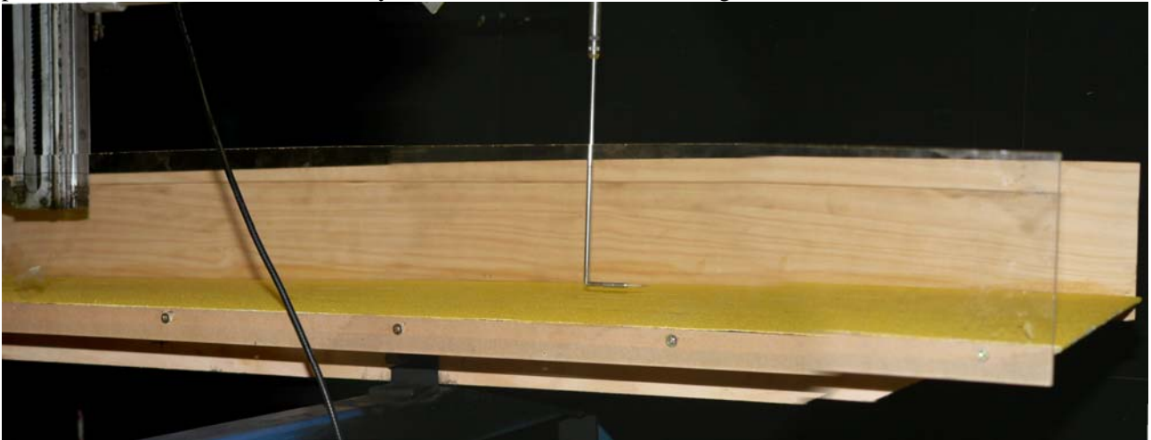
Fig. 2-2 - Photograph of the boundary layer experiment: rough plate (sand paper grade 40) - The hot-wire probe is located at x = +0.30 m and y = 0.010 m - Wind flow from right to left
