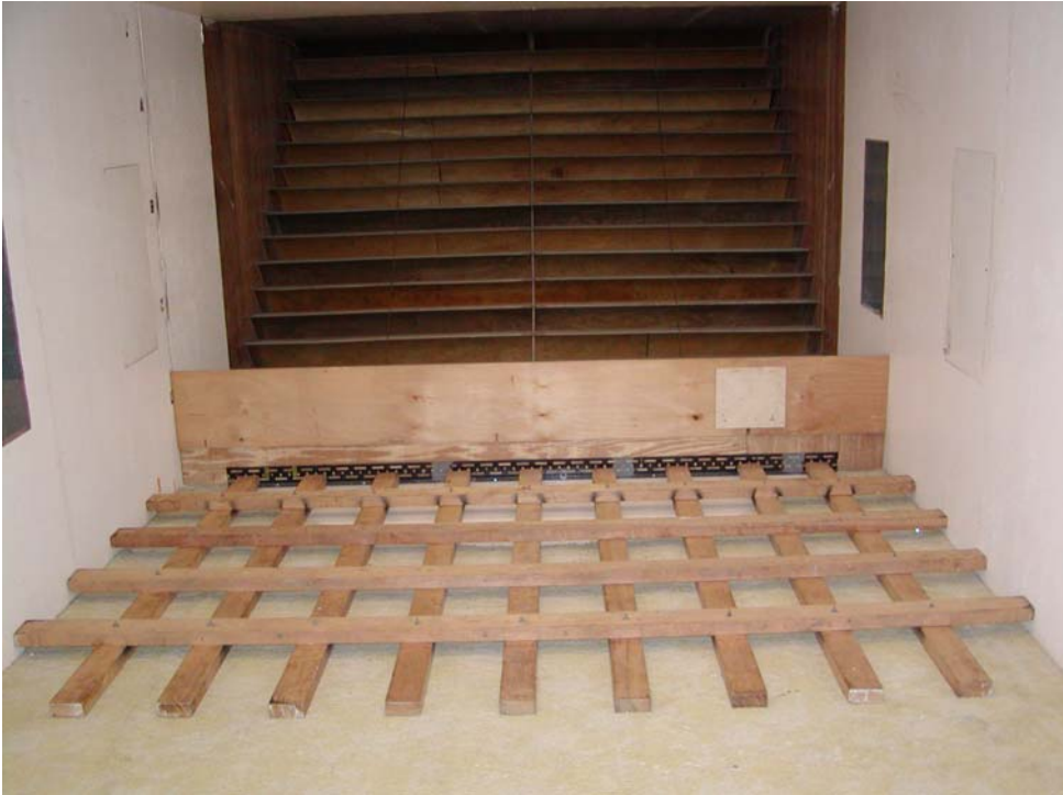
Fig. III-2 - Wind tunnel : downstream end
