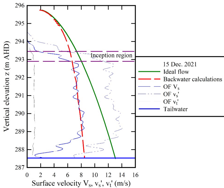
Fig. 8 Time-averaged OF surface velocity: comparison between time-averaged optical flow (OF) surface velocity data, ideal fluid flow velocity and backwater calculations at Chinchilla MEL weir
