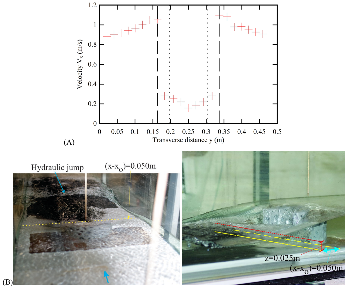
Figure 6. Transverse profile of longitudinal velocity at (x-x_0) = 0.050 m and z = 0.025 m for Q = 0.020 m 3 /s, d_1 = 0.10 m, porous Model L4 (Channel B). Dashed and dotted black mark the downstream edges of the horseshoe element. (A) Velocity profile; (B) Photographs of the flow.
