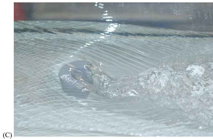
Figure 4. Flow patterns around a fully-submerged horseshoe element for d_1/H \sim 1.4 . (A) Model L4, d_1/H = 1.445 , Q = 0.0447 \text{ m}^3/\text{s} ; (B) Model M4, d_1/H = 1.38 , Q = 0.0121 \text{ m}^3/\text{s} ; (C) Model M1, d_1/H = 1.4 , Q = 0.0128 \text{ m}^3/\text{s} .
