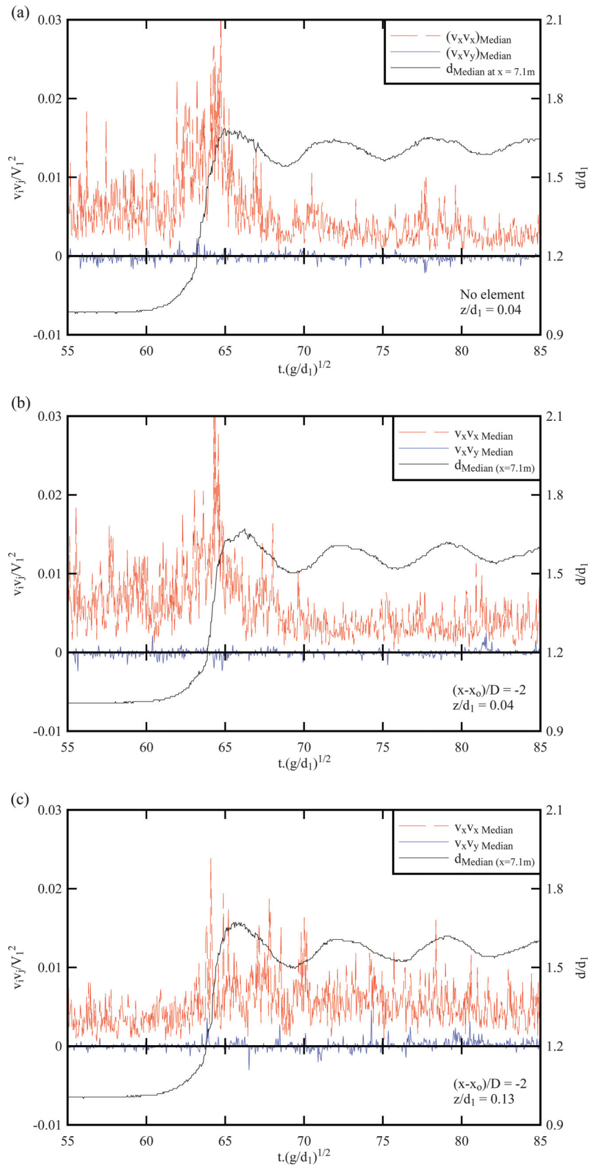
Fig. 10. Time variations of ensemble-averaged Reynolds stresses v_x v_x and v_x v_y ; comparison between bed configuration A (no element) and bed configuration B at (x - x_o)/D = -2 (upstream of large element) - Flow conditions: Q = 0.061 \text{ m}^3/\text{s} , d_1 = 0.155 \text{ m} at x = 5.9 \text{ m} , Fr_1 = 1.39 , y = 0 (centreline), Tainter gate opening after closure: h = 25 \text{ mm} . (a) Bed configuration A (no element), z/d_1 = 0.04 . (b) Bed configuration B at (x - x_o)/D = -2 , z/d_1 = 0.04 . (c) Bed configuration B at (x - x_o)/D = -2 , z/d_1 = 0.13 . [Colour online.]
