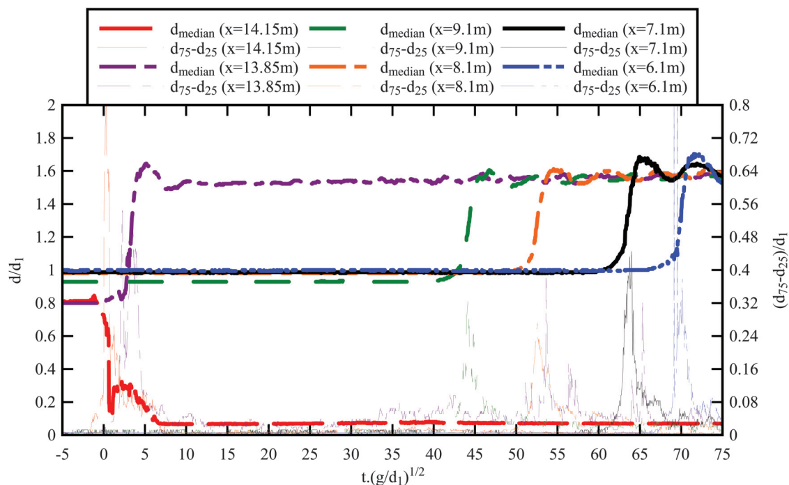
Fig. 7. Time variations of median water depth d_{\text{median}} and instantaneous free-surface fluctuations (d_{75} - d_{25}) during the generation and upstream propagation of a breaking bore — flow conditions: Q = 0.061 \text{ m}^3/\text{s} , d_1 = 0.155 \text{ m} at x = 5.9 \text{ m} , Fr_1 = 1.39 , x = 7.1 \text{ m} , y = 0 (centreline data), no roughness element, Tainter gate opening after closure: h = 25 \text{ mm} . [Colour online.]
