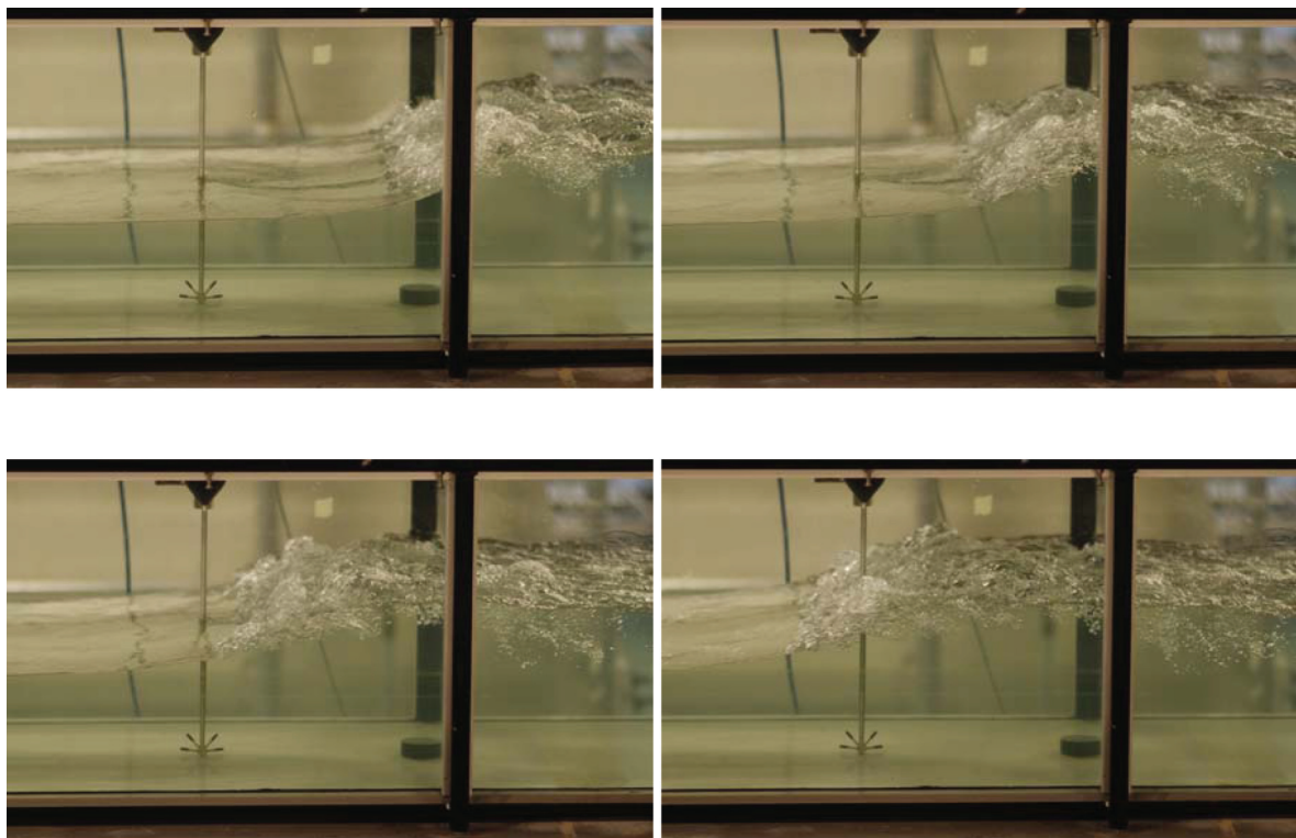
Fig. 3. Photographic sequence of tidal bore propagation (from right to left) with 0.12 s between successive photographs (from left to right, top to bottom) — flow conditions: Q = 0.061 \text{ m}^3/\text{s} , d_1 = 0.155 \text{ m} at x = 5.9 \text{ m} , Fr_1 = 1.39 , Tainter gate opening after closure: h = 25 \text{ mm} , shutter speed: 1/400 \text{ s} . [Colour online.]
