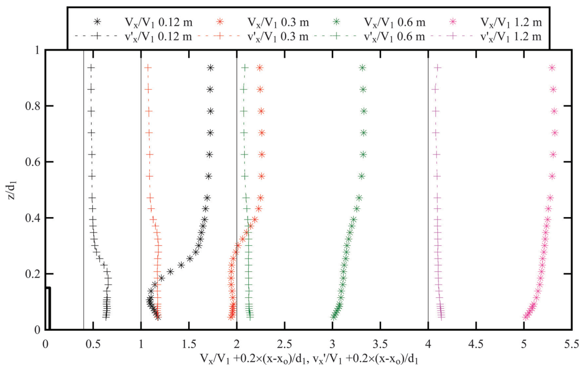
Fig. 4. Dimensionless vertical distributions of time-averaged longitudinal velocity V_x and standard deviation of longitudinal velocity v'_x downstream of the cylindrical element in steady flow — flow conditions: Q = 0.038 \text{ m}^3/\text{s} , d_1 = 0.130 \text{ m} at x = 5.9 \text{ m} , flow direction from left to right. Note the large cylindrical element drawn with a thick solid line on bottom left. [Colour online.]
