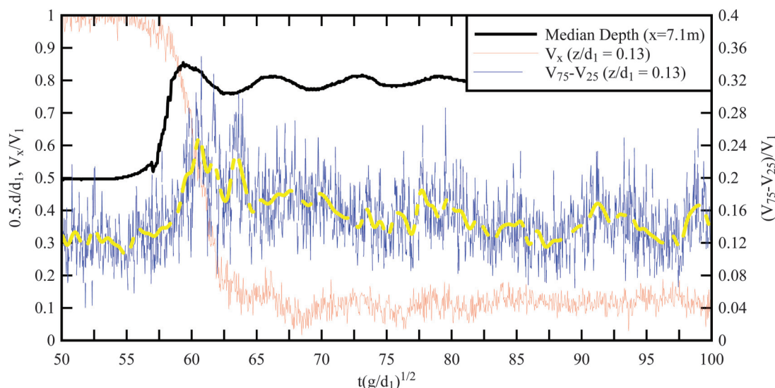
Fig. 9. Time variations of median water depth d_{\text{median}} , median longitudinal velocity V_x and instantaneous longitudinal fluctuations (V_{75} - V_{25}) during a breaking bore passage — flow conditions: Q = 0.061 \text{ m}^3/\text{s} , d_1 = 0.155 \text{ m} at x = 5.9 \text{ m} , Fr_1 = 1.39 , (x - x_o)/D = -2 , y/D = -0.5 , z/d_1 = 0.13 , Tainter gate opening after closure: h = 25 \text{ mm} . [Colour online.]
