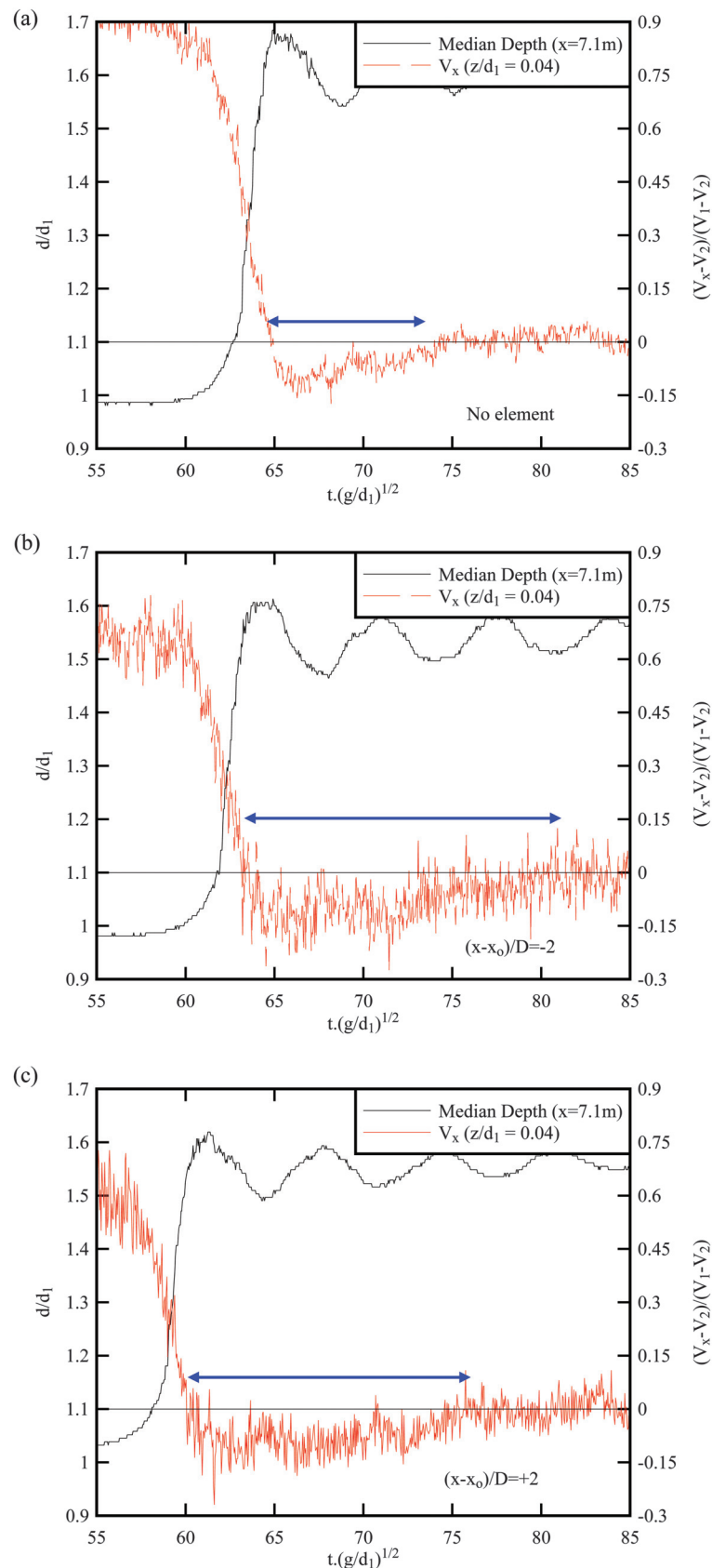
Fig. 8. Ensemble-averaged longitudinal velocity as a function of time: comparison between bed configuration A (no element) and bed configuration (with element) — flow conditions: Q = 0.061 \text{ m}^3/\text{s} , d_1 = 0.155 \text{ m} at x = 5.9 \text{ m} , Fr_1 = 1.39 , z/d_1 = 0.04 , y = 0 (centreline), Tainter gate opening after closure: h = 25 \text{ mm} ; blue arrow marks transient recirculation. (a) Bed configuration A (no element). (b) Bed configuration B: (x - x_o)/D = -2 (i.e., upstream of large element). (c) Bed configuration B: (x - x_o)/D = +2 (i.e., downstream of large element). [Colour online.]
