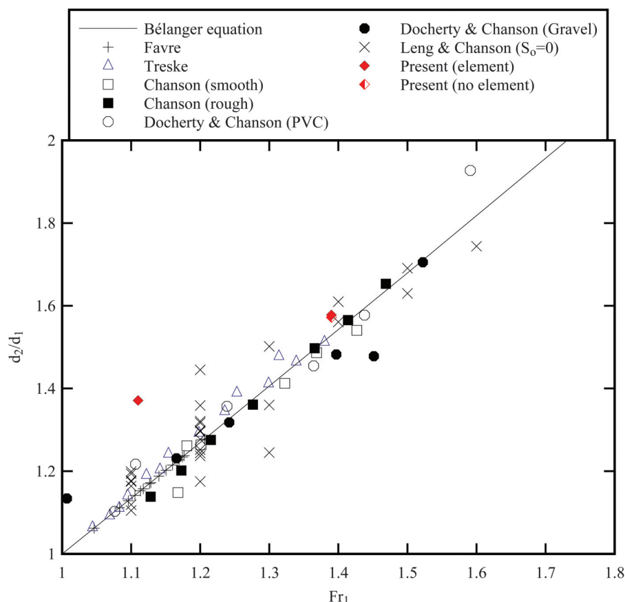
Fig. 5. Ratio of conjugate depths in tidal bores propagating in a horizontal rectangular channel. Comparison between present ensemble-averaged data at x = 7.1 m with and without large element and laboratory data on smooth invert (Favre 1935; Treske 1994; Chanson 2010a; Docherty and Chanson 2012; Leng and Chanson 2016) and rough invert (Chanson 2010a; Docherty and Chanson 2012). [Colour online.]
