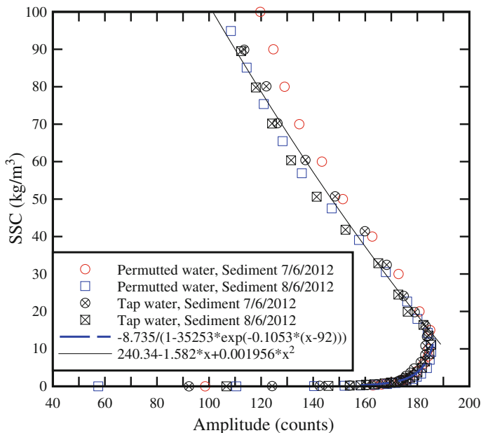
Fig. 9 Relationship between suspended sediment concentration and acoustic signal amplitude with the sediment samples collected at Arcins—comparison between the data and Eqs. (9) and (10)
