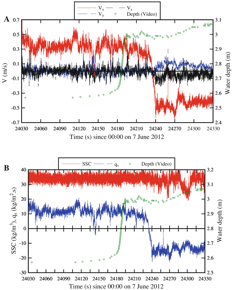
Fig. 7 Details of the time variations of the flow and sediment properties in the tidal bore of the Garonne River on 7 June 2012 morning. a Time variations of the water depth and turbulent velocity components in the tidal bore of the Garonne River on 7 June 2012 morning. b Time variations of the water depth, sediment concentration estimate and longitudinal sediment flux in the tidal bore of the Garonne River on 7 June 2012 morning
