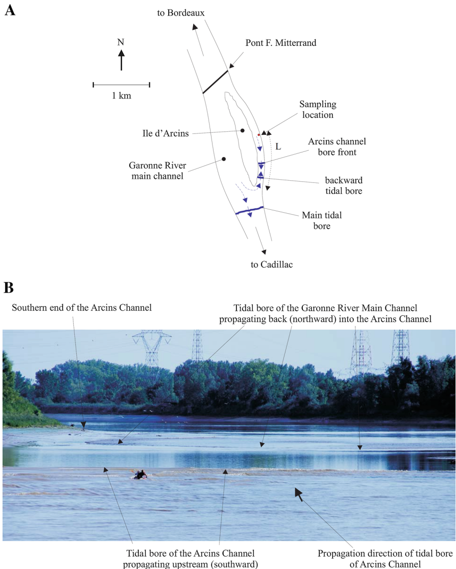
Fig. 8 Tidal bore of the Garonne River main channel entering the southern end of the Arcins channel and propagating northwards against the tidal bore of the Arcins channel. a Sketch of the tidal bore of the Garonne River main channel entering into the southern end of the Arcins channel and propagating northwards against the flood flow in the Arcins channel. b Photographic observation on 22 August 2013 looking south towards the southern end of the Arcins channel
