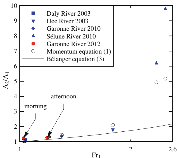
Fig. 4 Dimensionless relationship between the conjugate cross-sectional area ratio A_2/A_1 and tidal bore Froude number Fr_1 —comparison between the present field data, Eq. (1), the Bélanger equation (Eq. 3), and the data of Wolanski et al. [45] (Daly River), Simpson et al. [40] (Dee River), Mouaze et al. [34] (Sélune River) and Chanson et al. [5,6] (Garonne River)
