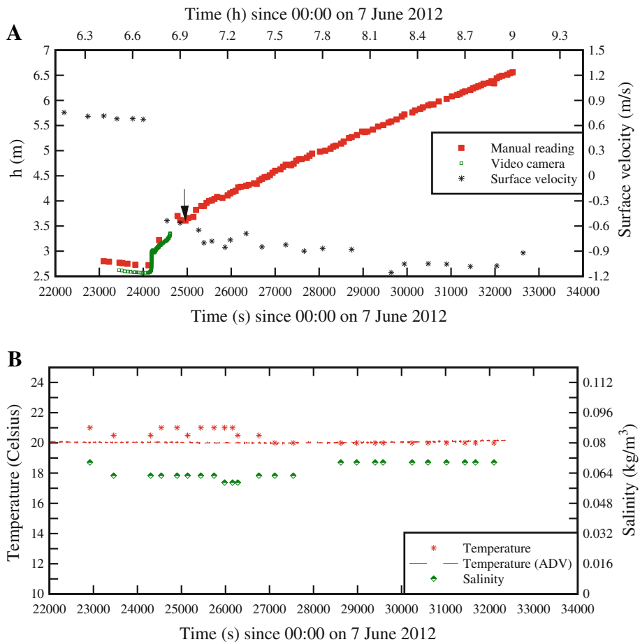
Fig. 5 Time-variations of the water depth, free-surface velocity, water temperature, salinity, longitudinal and transverse velocity component (ADV data), suspended sediment concentration, and longitudinal sediment flux on 7 June 2012 morning in Arcins about the tidal bore passage. a Water depth next to the ADV unit, b water temperature and salinity, c longitudinal and transverse velocity component (ADV data), and d suspended sediment concentration estimate and longitudinal suspended sediment flux
