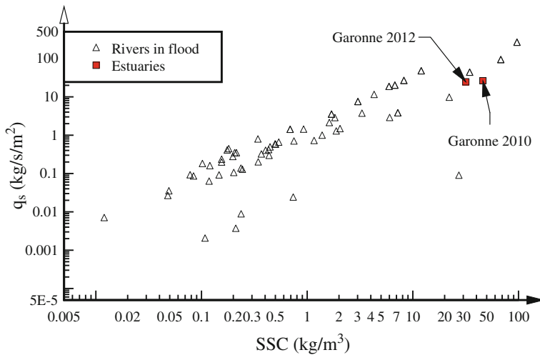
Fig. 10 Suspended sediment flux q_s ( \text{kg s}^{-1} \text{m}^{-2} ) as function of the suspended sediment concentration SSC—comparison between present data (Garonne 2012), the 2010 observations (Garonne 2010) together with observations in rivers during floods (Amazon, Brisbane, Fitzroy, Huanghe, Mississippi, Nile, North Fork Toutle, Rio Puerco)
