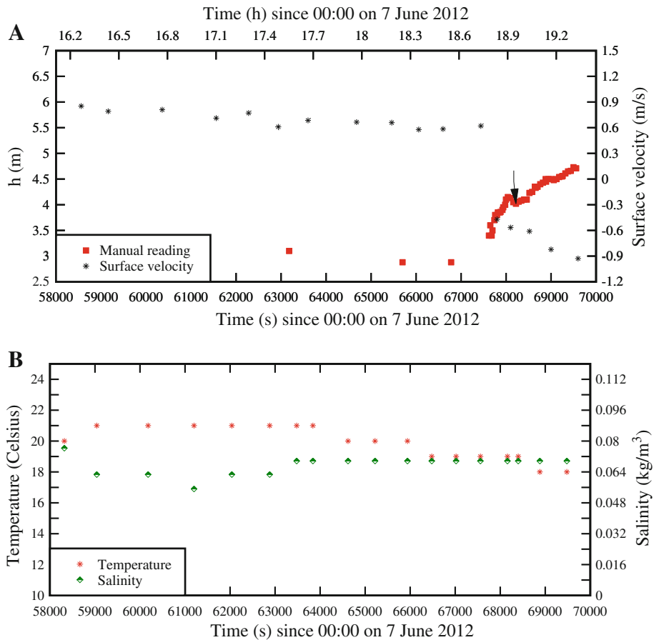
Fig. 6 Time-variations of the water depth, free-surface velocity, water temperature and salinity on 7 June 2012 afternoon in Arcins about the tidal bore passage. a Water depth next to the ADV unit and b water temperature and salinity
