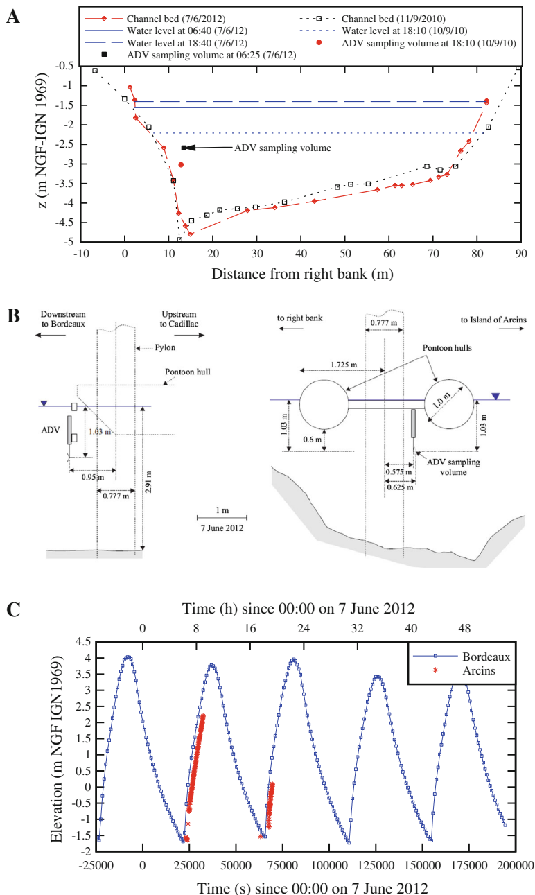
Fig. 3 Arcins channel cross-section and observed water levels. a Surveyed cross-section of Arcins channel looking upstream with the low tide water level on 7 June 2012 afternoon and the corresponding ADV sampling volume location—comparison between the 2010 and 2012 surveys at the same cross-section. b Un-distorted sketch of the ADV mounting, sampling volume location and water surface 20 min prior to the tidal bore on 7 June 2012 morning: left view from Arcins Island, right looking upstream. c Measured water elevations in the Arcins channel on 7 June 2012 and in Bordeaux ( 44^{\circ}52'N , 0^{\circ}33'W ) (Data Vigicrue, Ministère de l'Environnement et du Développement Durable)
