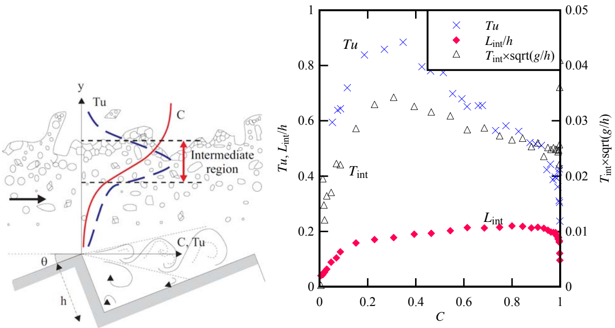
Figure 9 Air-water skimming flow on a stepped spillway: the intermediate region ( 0.3 < C < 0.7 ) - Experimental data: Felder and Chanson (2009), \theta = 21.8^\circ , h = 0.05 m, d_c/h = 2.39 , \rho_w q_w / \mu_w = 1.3 \times 10^5 , step edge 18
